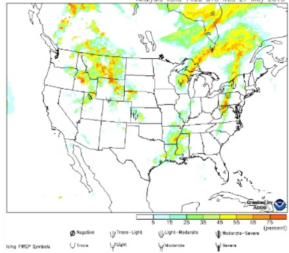
Maximum icing probability (1000 ft. MSL to FL300) Analysis valid 1400 UTC Wed 27 May 2015
