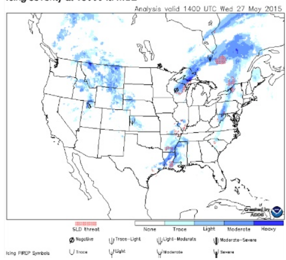
Icing severity at 15000 ft. MSL Analysis valid 1400 UTC Wed 27 May 2015
