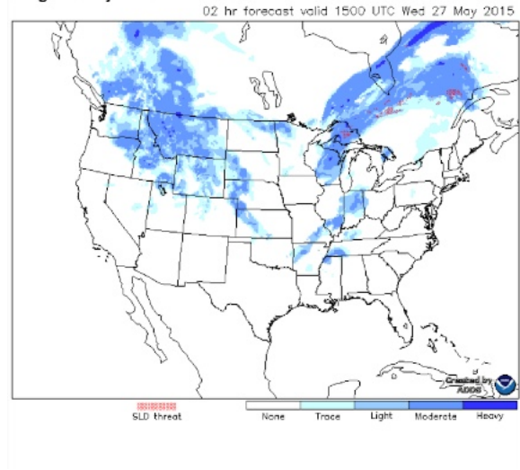
Icing severity at 13000 ft. MSL
